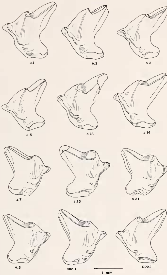
Fig. 2. Crocidura suaveolens canae , P 4 , Kommos, sample nos. indicated below the teeth.
